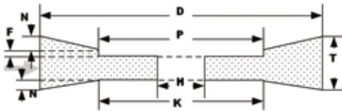
Form 26: Double-sided tapered, double-sided recessed grinding wheel D \times T/N \times H - P \times F/G
