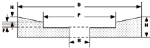
Form 24: Double-sided recessed, single-sided tapered grinding wheel D \times T/N \times H - P \times F/G
